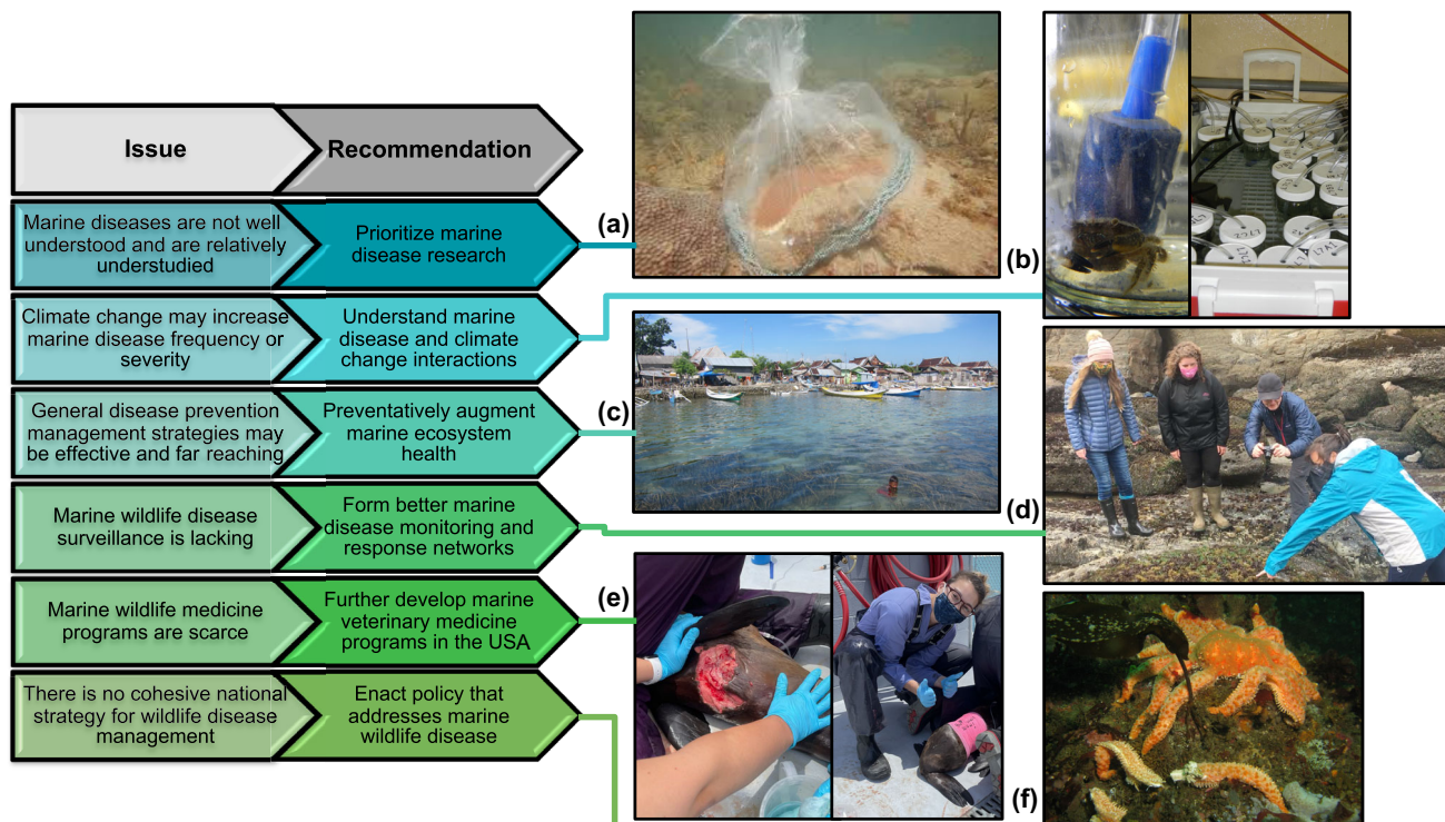
FIGURE 3 Issues in marine disease management and accompanying recommendations. (a) The CHAMP Laboratory (Coral Health and Marine Probiotics) of University of North Carolina Wilmington applies probiotics to corals off the coast of Florida, USA to treat stony coral tissue loss disease. Photograph by Hunter Noren. (b) Mesocosm infection experiments of the mud crab, Eurypanopeus depressus by parasitic barnacle Loxothylacus panopaei enable incorporating mechanistic environmental response in epidemiological models (Gehman et al., 2018). Photograph by Alyssa Gehman. (c) Restoration and conservation of sea grass bed habitats, which can act as natural ecosystem filters (Lamb, van de Water, Bourne, Altier, Hein, et al., 2017). (d) Members of the PRIMED Network training volunteers to identify and report marine diseases using iNaturalist. Photograph by Sarah Gravem. (e) A veterinary medicine student at Oregon State University treating a wound on an injured sea lion. Photograph Robyn Cates. (f) The Endangered Species Act is being used to help species recover from sea star wasting disease, yet there is no explicit policy managing wildlife disease. Photograph by Janna Nichols in Washington, USA
