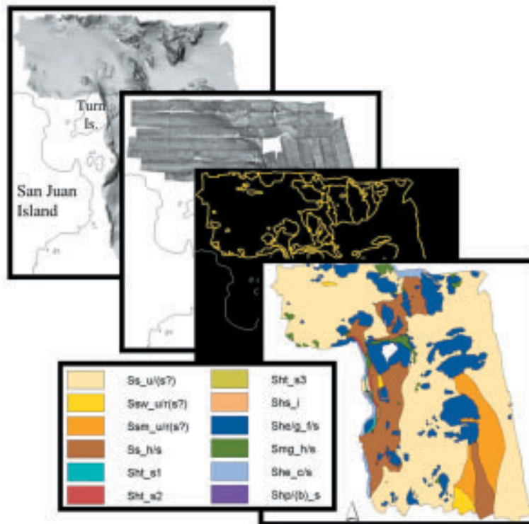
Figure 3.10. Example of nested data layers used in the compilation and construction of maps of potential marine benthic habitats. Locality is San Juan Channel offshore of San Juan Island, Washington. 3.10a = multibeam bathymetry; 3.10b = multibeam backscatter; 3.10c = line drawing of interpreted habitat types; 3.10d= potential habitat polygons. Refer to Appendix 3.1 for explanation of habitat code.
